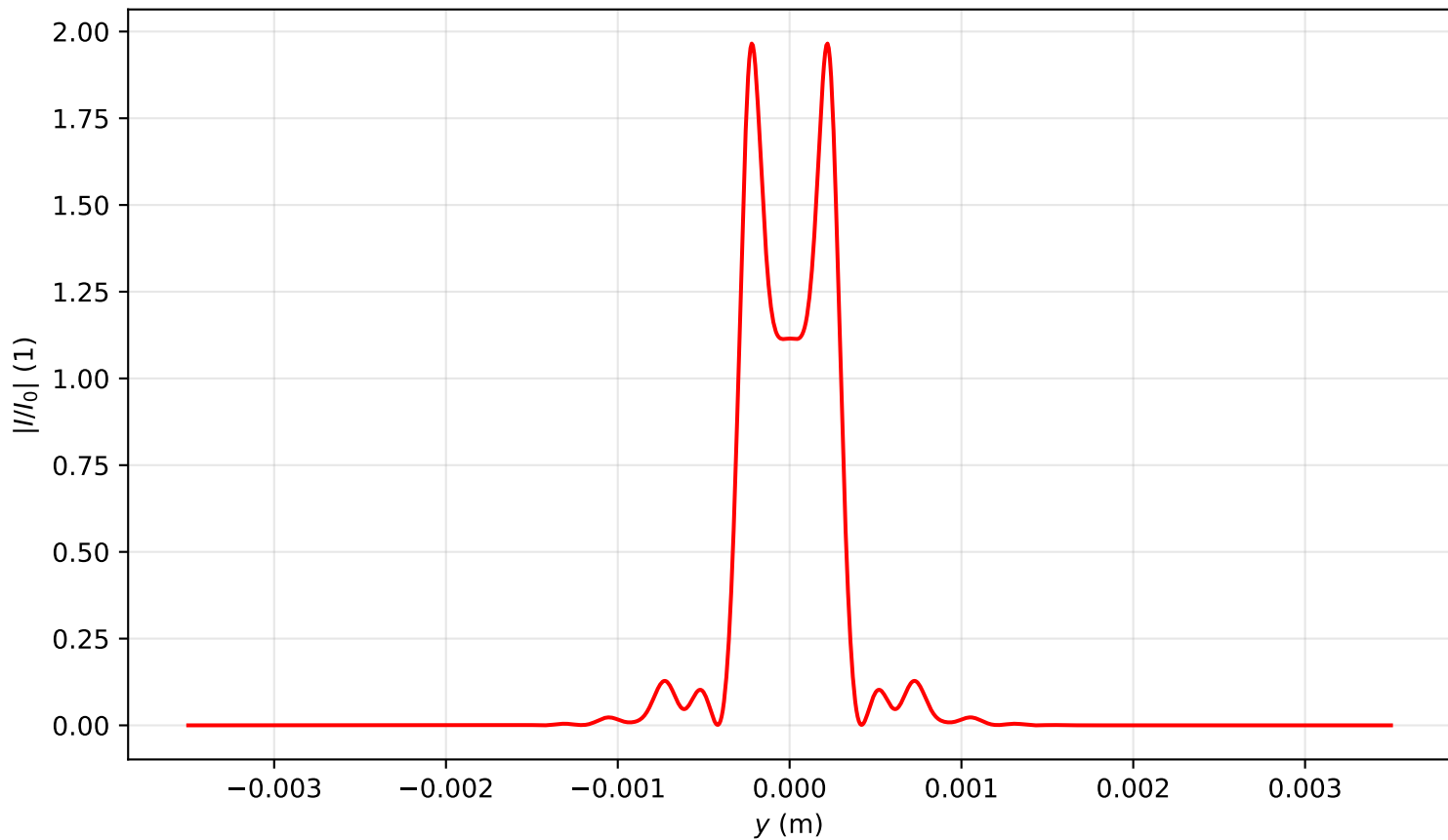
Intensity profile I(x = 0, y, z = 0.716)/I_0 , P_{in}=7.0P_{cr} , artificial time
